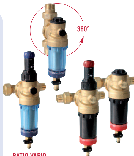
RATIO VARIO Compact backwash filter like RATIO plus rotatable flange for vertical and horizontal installation
